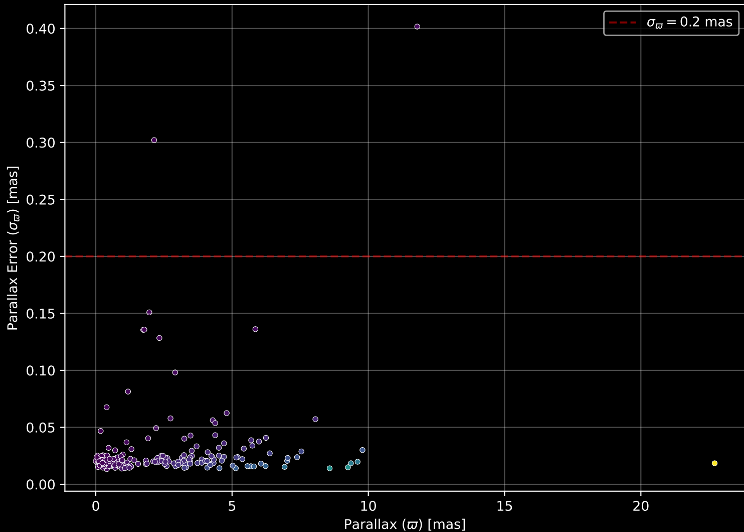
APOGEE DR17 Field: [K2_C6_325+49_btx] Parallax Quality (n= 186)
