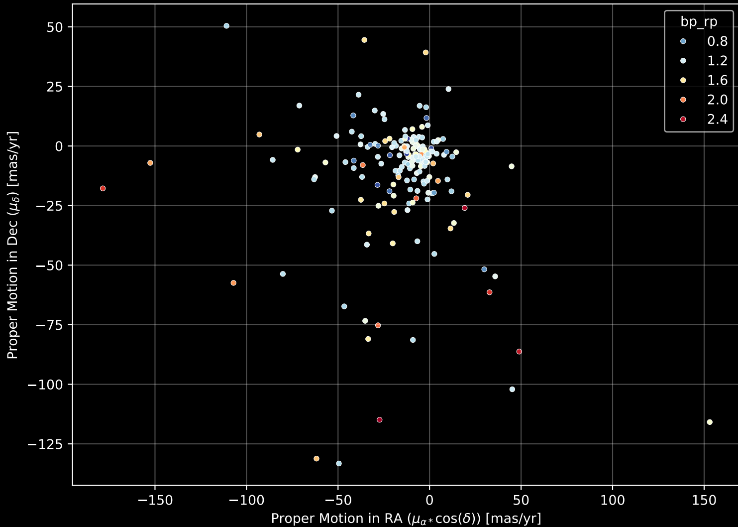
APOGEE DR17 Field: [K2_C6_325+49_btx] Proper Motion Diagram (n= 186)
