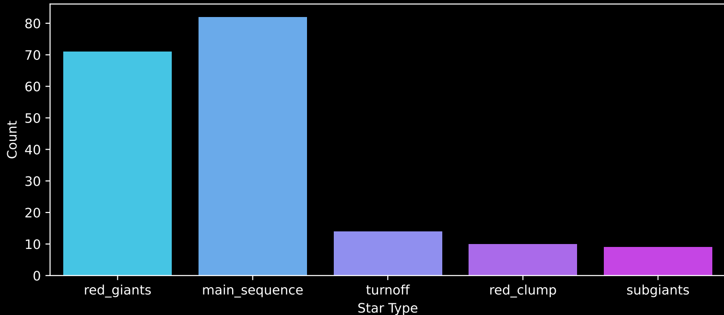
APOGEE DR17 Field: [K2_C6_325+49_btx] Count plot of Star Type
