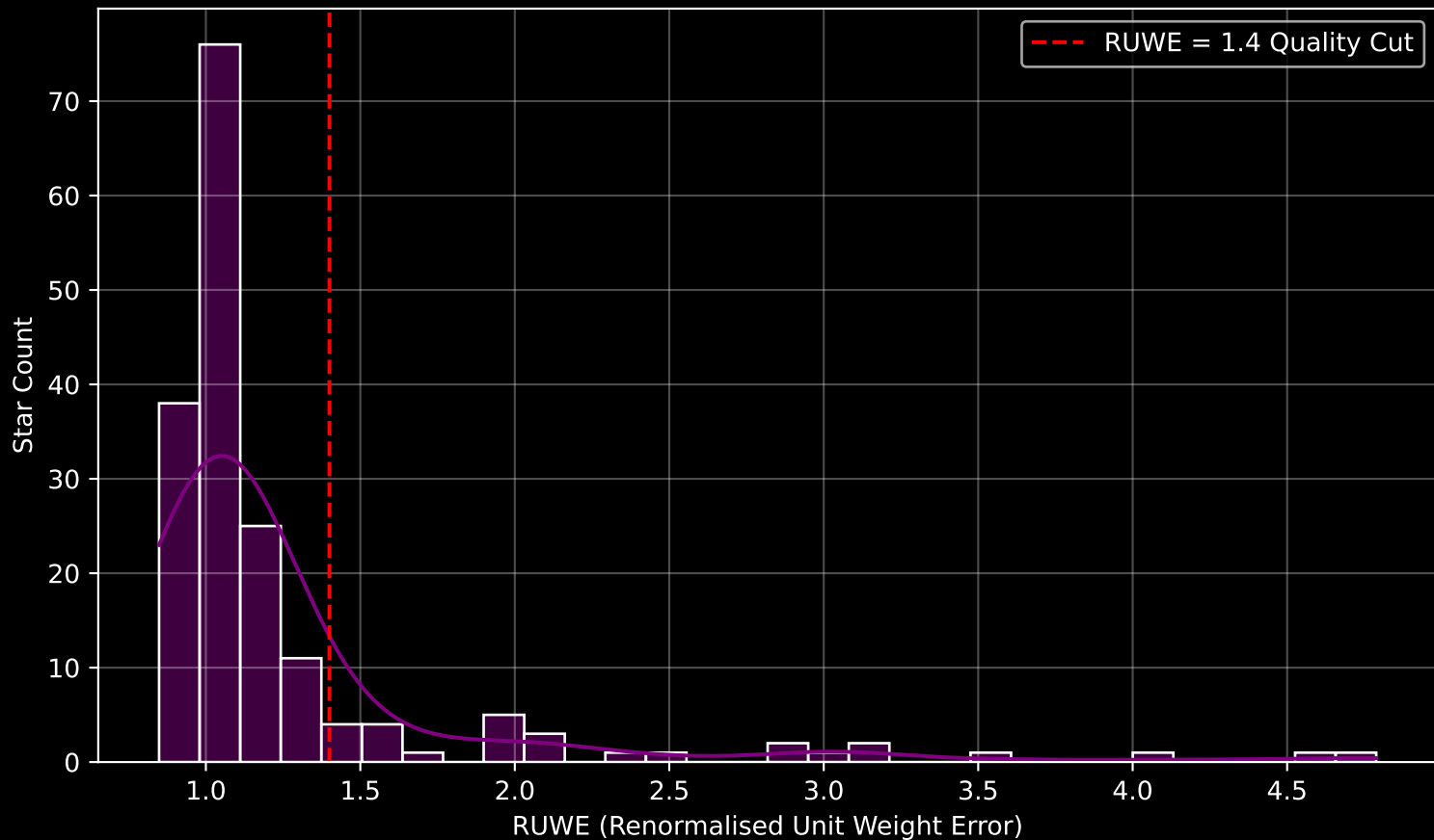
GAPOGEE DR17 Field [K2_C6_325+49_btx] RUWE Distribution (n= 178)
