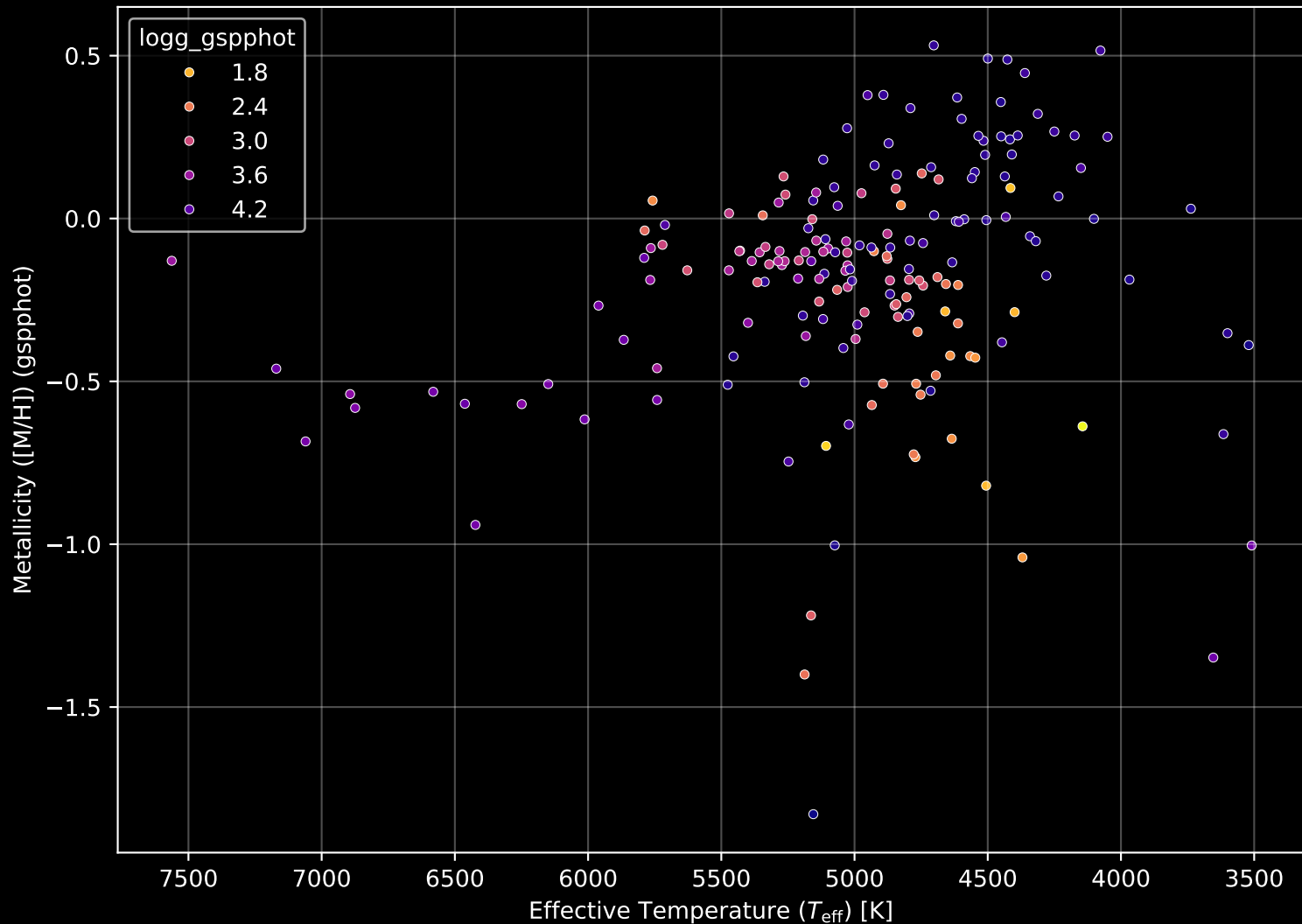
APOGEE DR17 Field: [K2_C6_325+49_btx] Stellar Population Parameters (n= 186)
