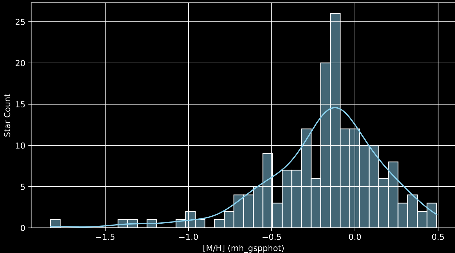
APOGEE DR17 Field: [K2_C6_325+49_btx [M/H] (mh_gspphot) (n= 184)
